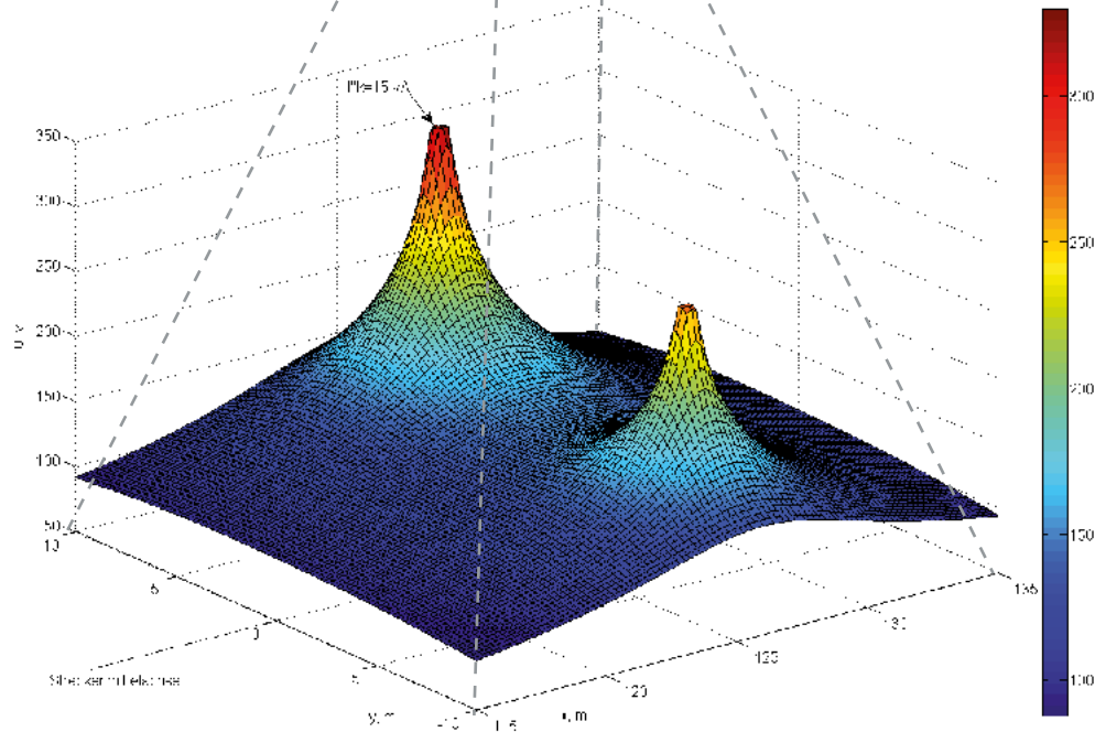
Earth surface potential in the event of a short-circuit due to flashover of an insulator on mast 5.
