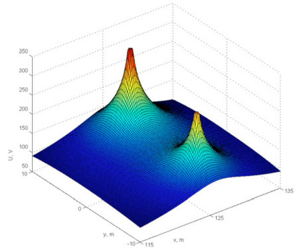
Earth surface potential in the event of a short-circuit due to a flashover of an insulator on the mast
