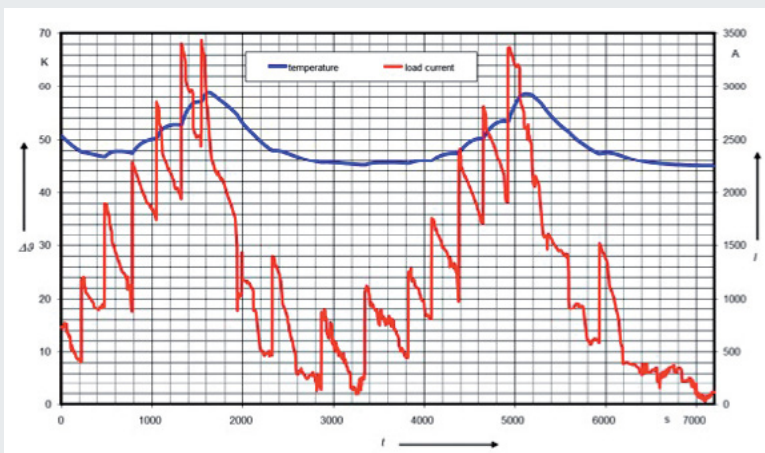
Temperature profile and load current of an overhead contact line
