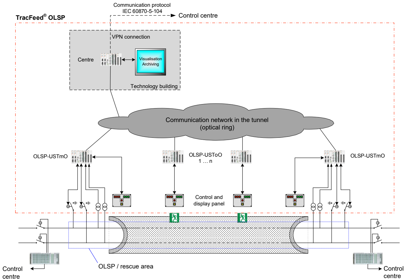
TracFeed® OLSP quick reference guide
