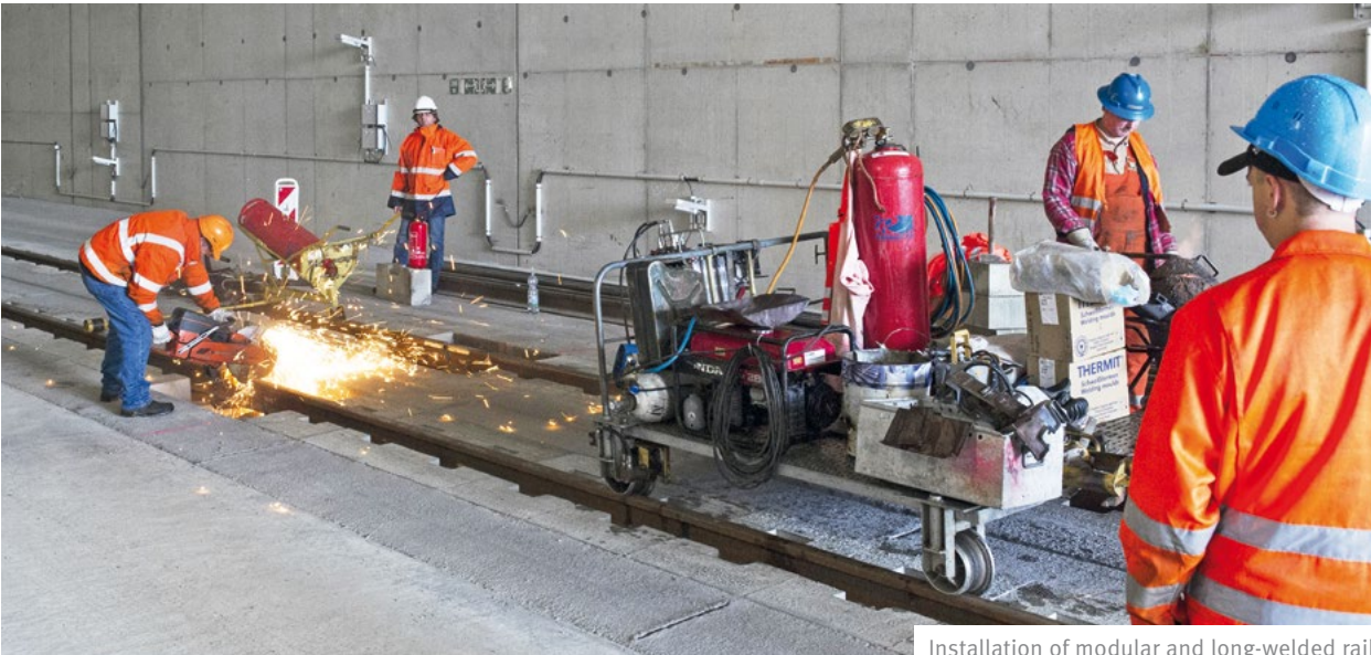
Installation of modular and long-welded rails
