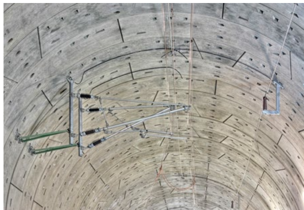
Support point with cantilever (push off)
